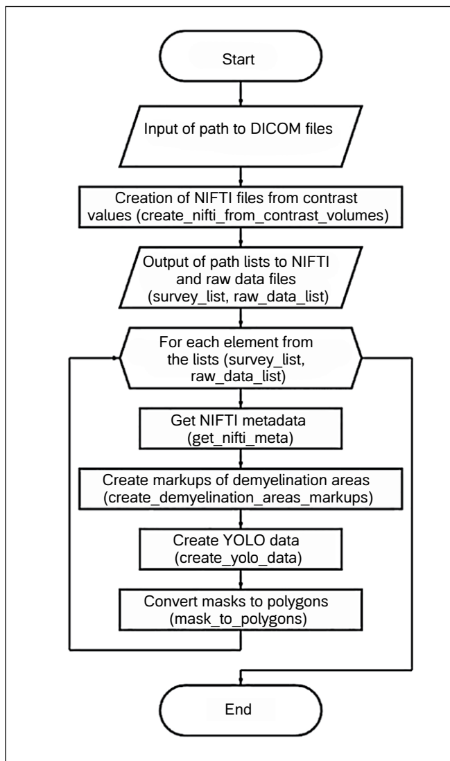
Figure 2. Flowchart of the algorithm for creating a training sample.
